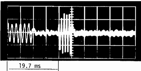
Figure 5. Oscilloscope display showing leading edge of WWV tick at a sweep rate of 5 ms/division
