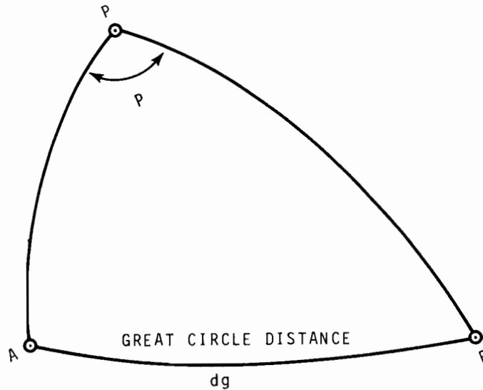
Figure 23. Diagram for great circle distance calculations.
