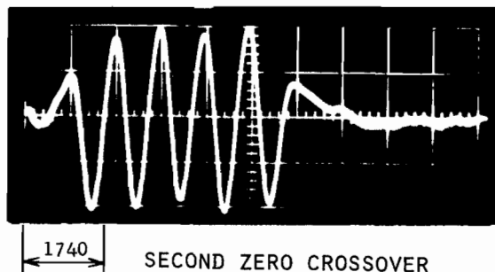
Figure 8. Oscilloscope display showing second zero crossover of WWV tick at a sweep rate of 1 ms/division
