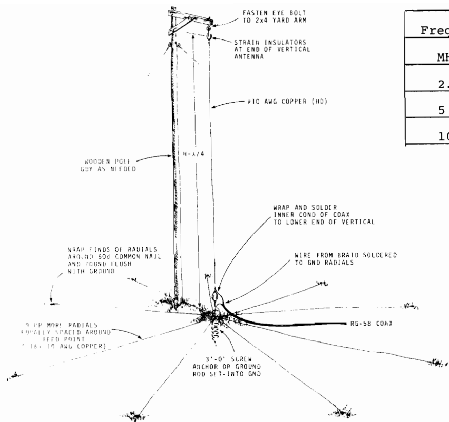
Figure 18. Quarter-wavelength vertical antenna & horizontal half-wavelength antenna.
