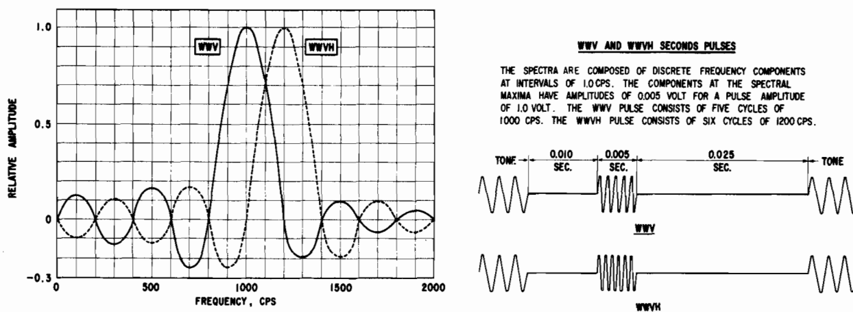
Figure 1. WWV and WWVH seconds pulses.
