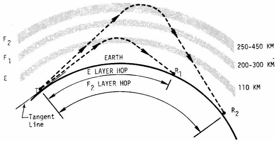
Figure 24. Reflection of radio waves at different ionized layer heights.
