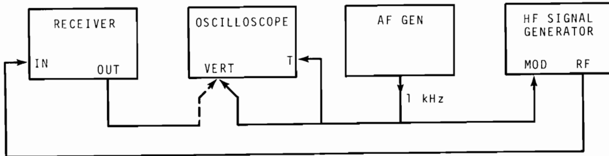
Figure 21. Equipment setup for receiver time delay measurements.
