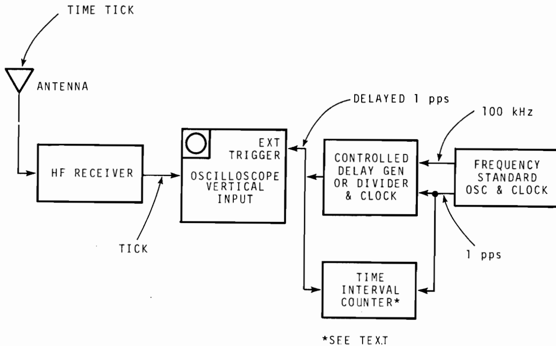
Figure 7. Equipment setup for delayed trigger method of time synchronization.
