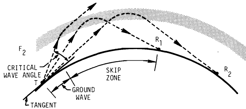
Figure 26. Single-hop transmission at different wave angles.
